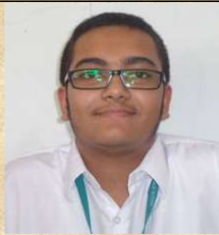
SHIVANQ DALAL (95.8%)
